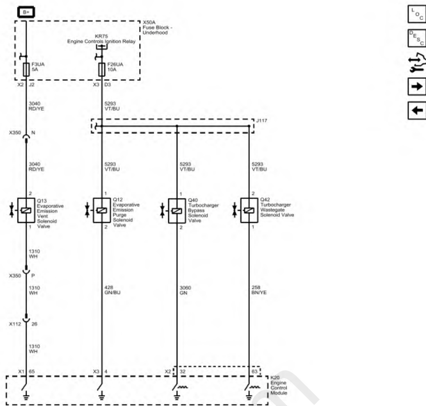
Fig. 10: Fuel Controls - Evaporative Emission and Device Controls (Buick with LE2) Courtesy of GENERAL MOTORS COMPANY
