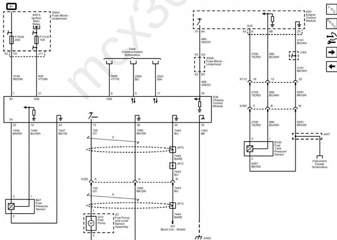
Fig. 11: Fuel Controls - Fuel Pump and Fuel Pump Controls (Buick with LE2) Courtesy of GENERAL MOTORS COMPANY
