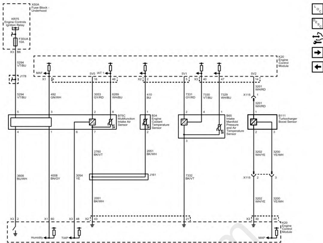
Fig. 4: Intake, Manifold, and Engine Coolant Sensors (Buick with LE2). Courtesy of GENERAL MOTORS COMPANY
