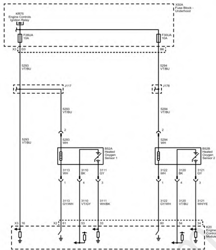
Fig. 8: Oxygen Sensors (Buick with LE2) Courtesy of GENERAL MOTORS COMPANY
