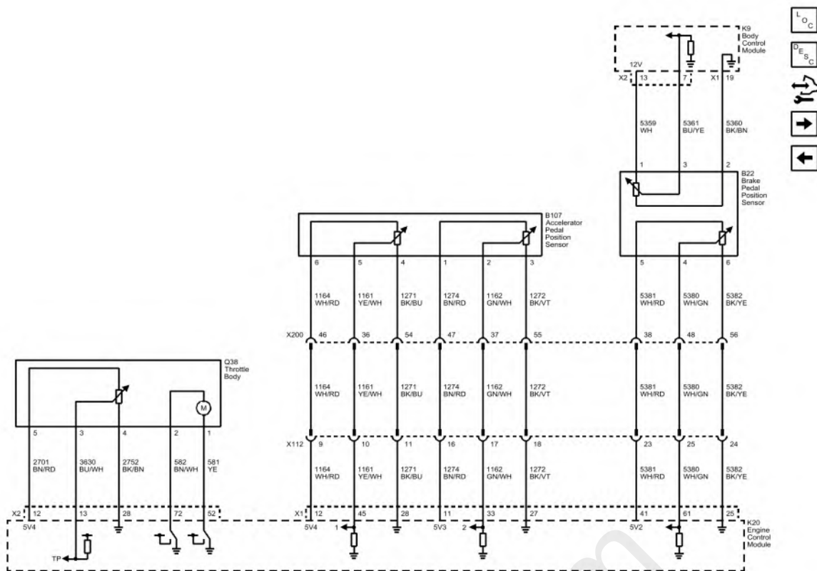
Fig. 6: Throttle Body, Accelerator Pedal Position Sensor, and Brake Pedal Position Sensor (Buick with LE2)
