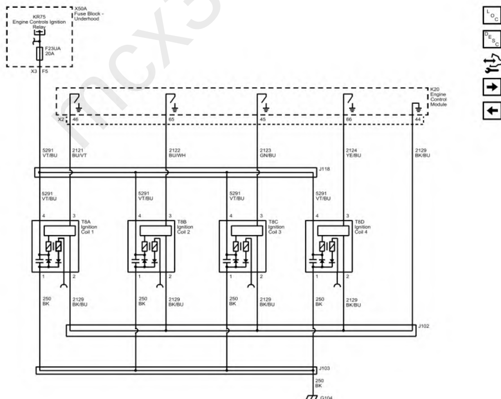
Fig. 7: Ignition Controls (Buick with LE2)
