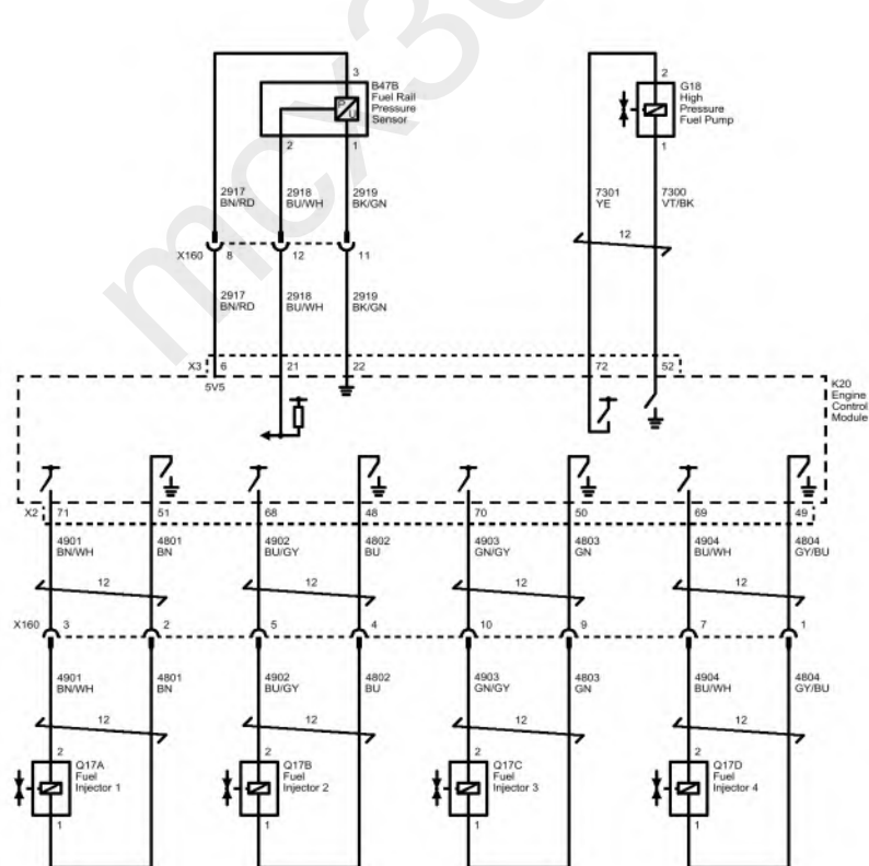
Fig. 9: Fuel Controls - Fuel Injectors and High Pressure Fuel Control (Buick with LE2) Courtesy of GENERAL MOTORS COMPANY
