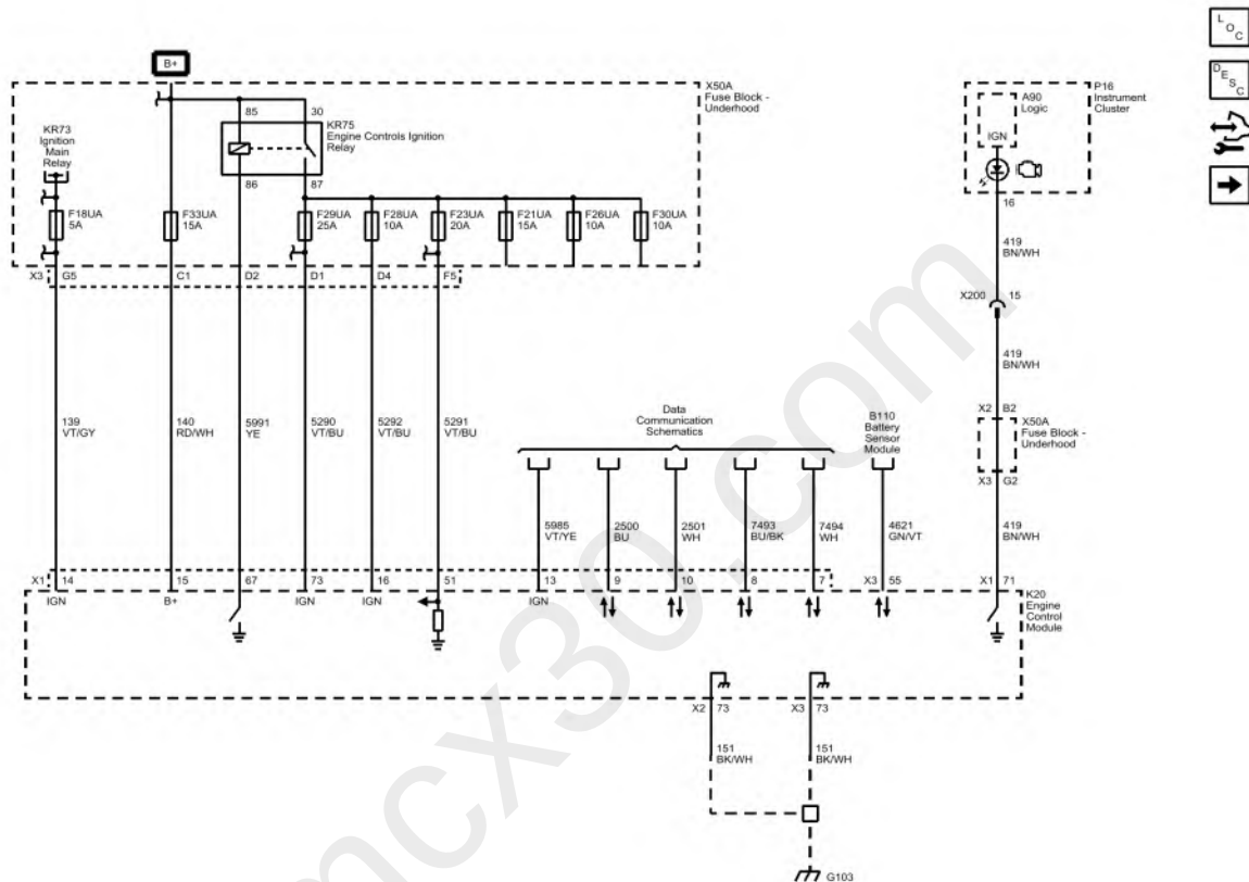
Fig. 1: Module Power, Ground, Serial Data, and MIL (Buick with LE2). Courtesy of GENERAL MOTORS COMPANY
